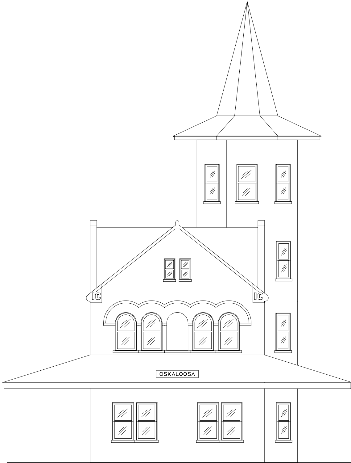
NORTH ELEVATION
